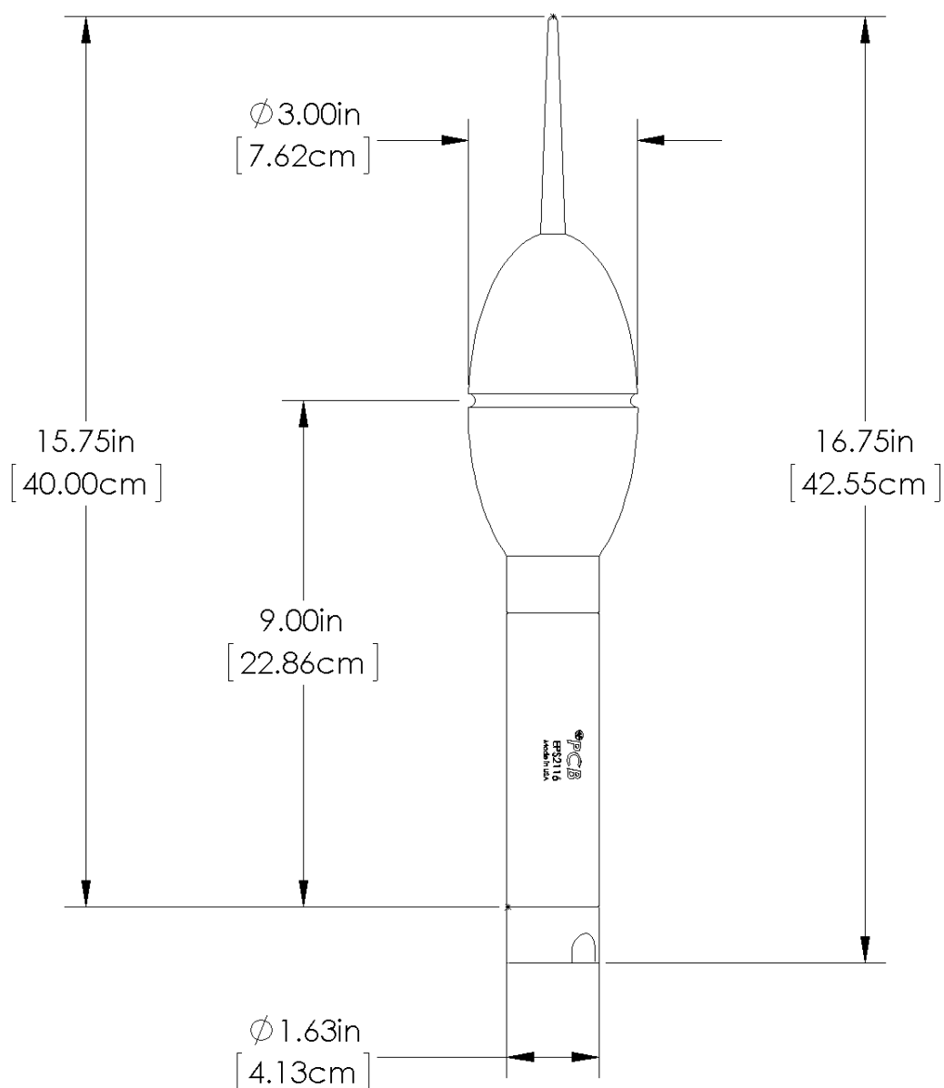
FIGURE A-1 EPS2116 Dimensions
