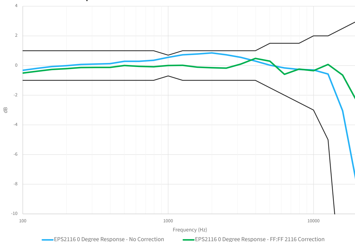
FIGURE A-5 EPS2116 Response at 0 °
