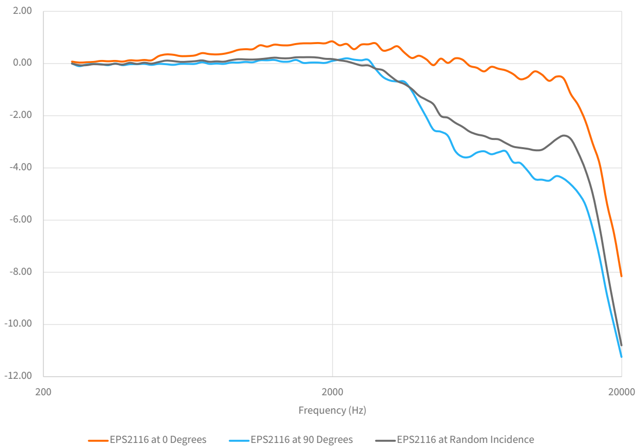
FIGURE A-3 Correction Factors for the EPS2116
