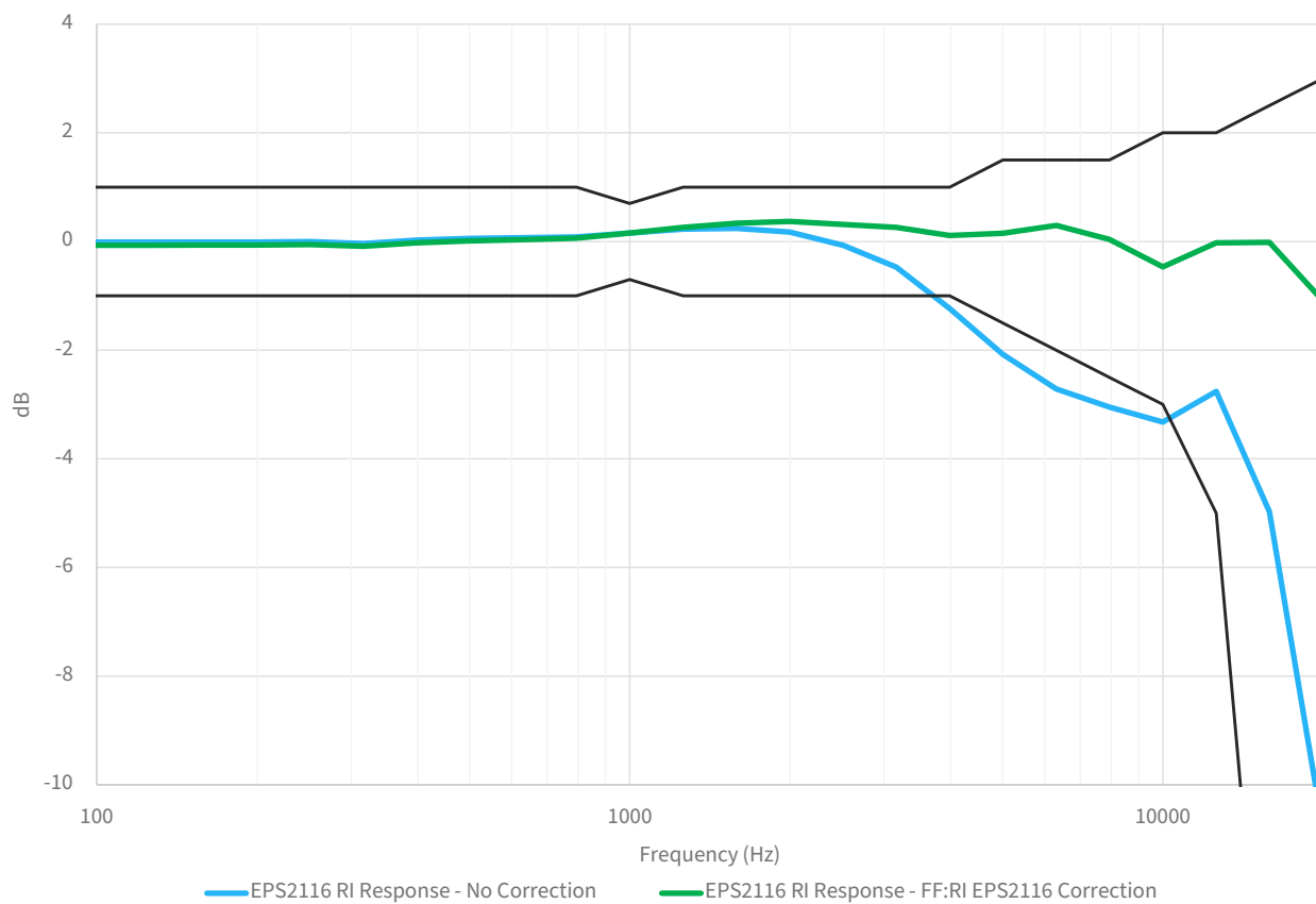
FIGURE A-7 EPS2116 Random Incidence Response
