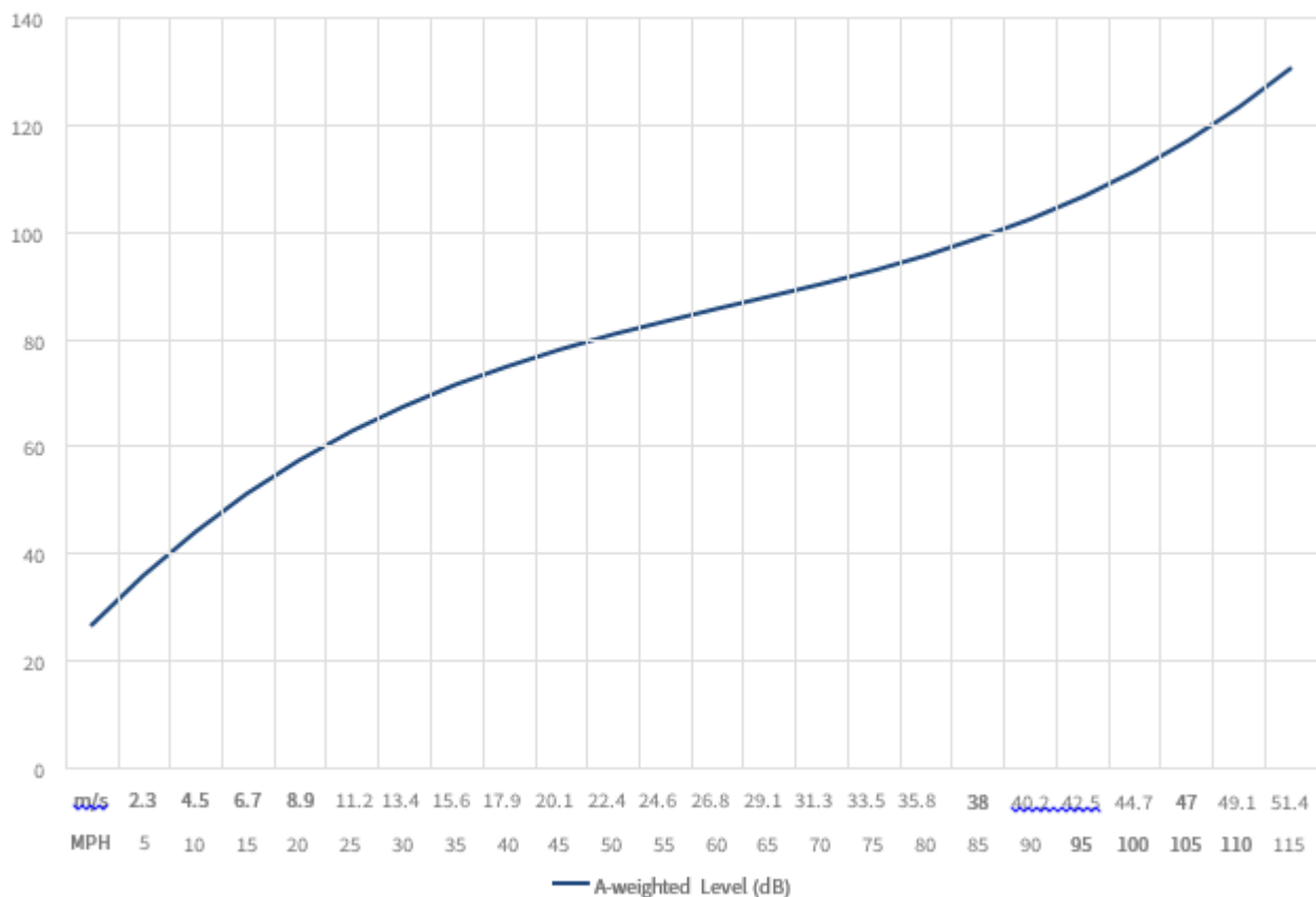
FIGURE A-2 Wind-Induced Noise Graph A-Weighted Level (dB)
