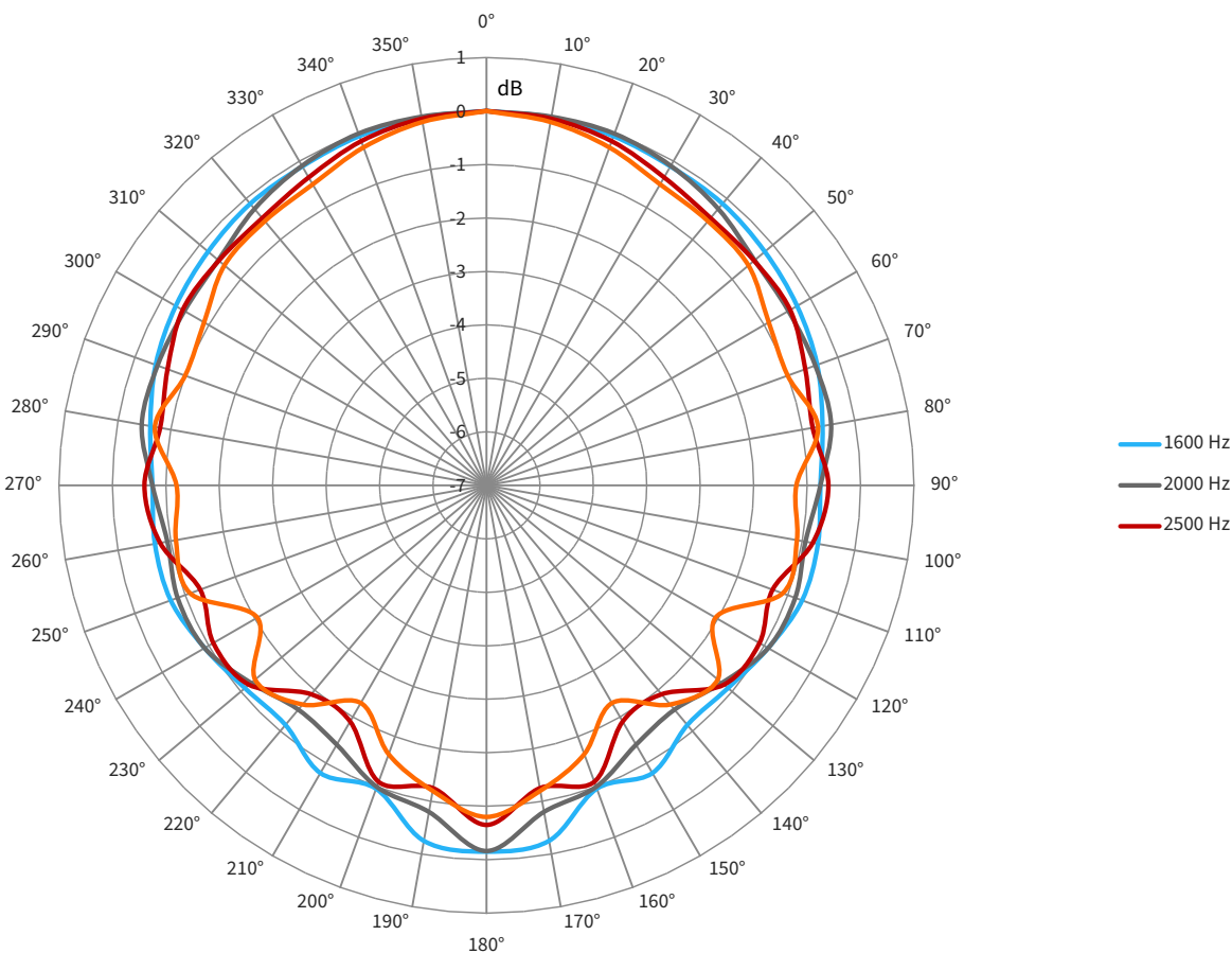
FIGURE A-9 EPS2116 Directional Response (1600 Hz–3150 Hz)
