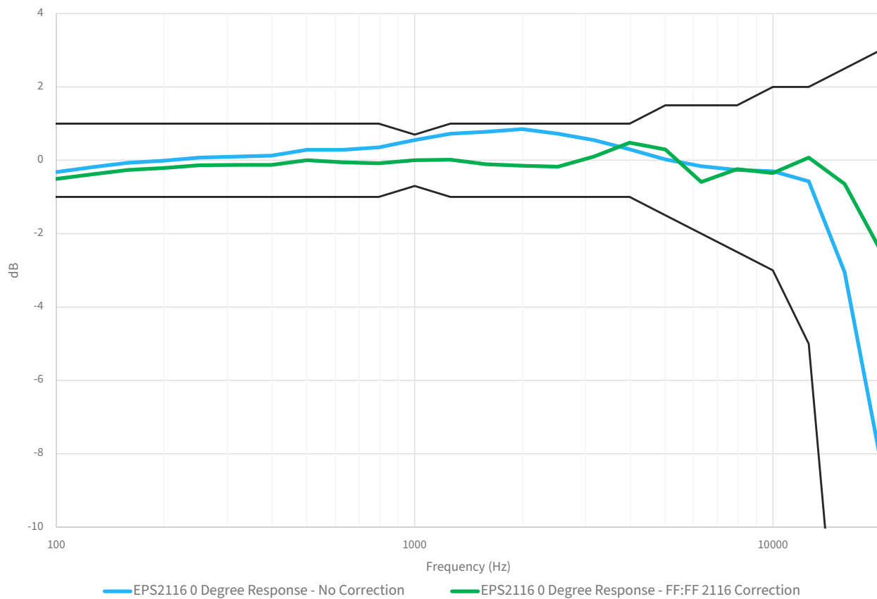
FIGURE A-6 EPS2116 Response at 90°
